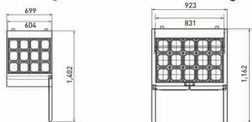
FMU-28
