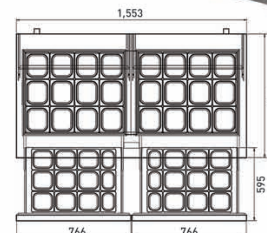
FMU-60-2D-4
