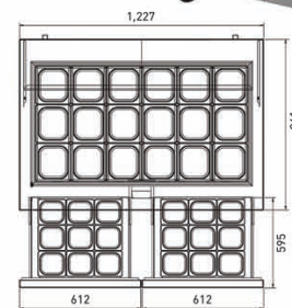
FMU-48-2D-4
